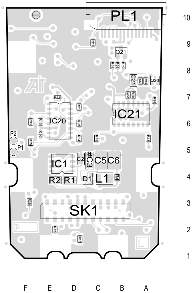
ORCA KEYPAD INTERFACE 220-01412-00 A BOTTOM COPPER
