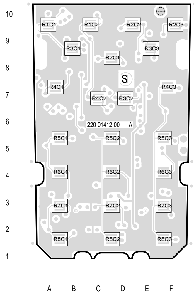
ORCA KEYPAD INTERFACE 220-01412-00 A TOP COPPER
